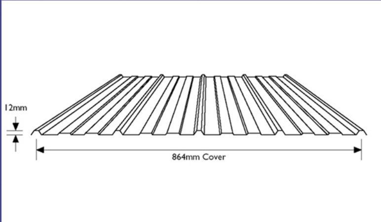
Stramit K Panel
