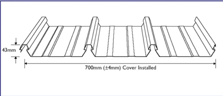
Stramit Speed Deck Ultra
