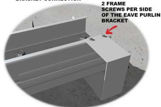
DOUBLE COLUMN EAVE PURLIN BRACKET CONNECTION
