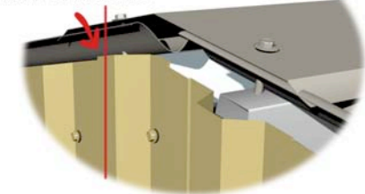
SCREWS AS PER ENGINEERING PLANS
