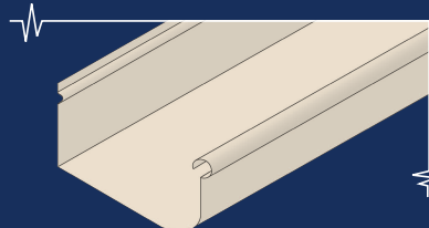
Stramit® Quad 115 / 125 Gutter Plain only
