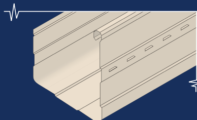
Stramit® M-Pattern Gutter Plain / Slotted
